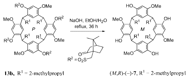
Scheme 14. Hydrolysis of the first eluting tetracamphorsulfonate derived from (R)\text{-}(-)\text{-10} -camphorsulfonyl chloride.
