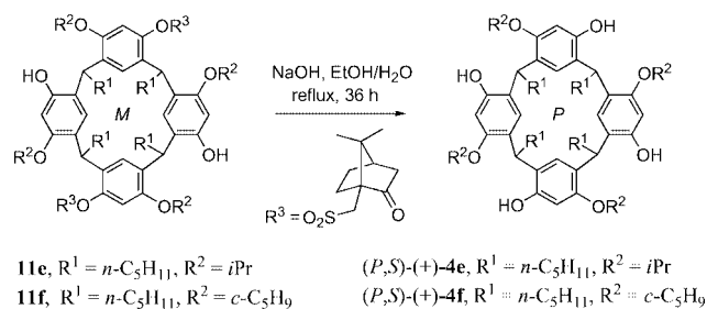
Scheme 13. Hydrolyses of the first eluting dicamphorsulfonates derived from ( S )-(+)-10-camphorsulfonyl chloride.
